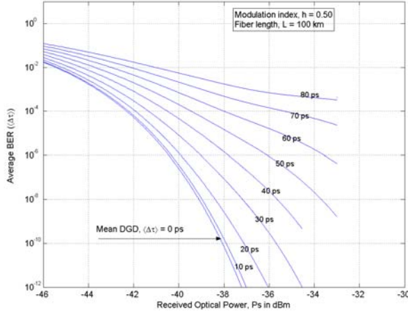
Fig. 2. Plots of average BER versus received power, P_s for heterodyne CPFSK receiver impaired by PMD at modulation index 0.50
