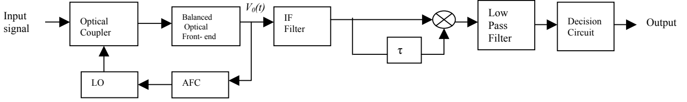
Fig.1. Block diagram of a heterodyne CPFSK delay demodulation receiver
