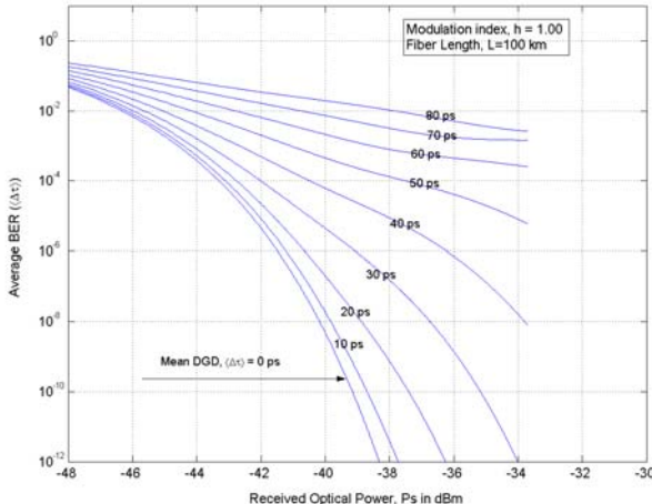
Fig. 3. Plots of average BER versus received power, P_s for heterodyne CPFSK impaired by PMD at modulation index 1.00
