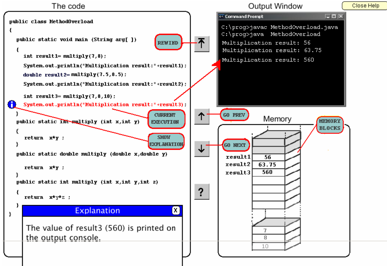
Fig.2: A typical e-Learning developed object (concept of method overloading in Java)
